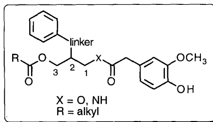
Templates as Simplified RTX Analogues
