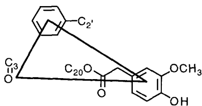
Proposed Pharmacophore Model of RTX
